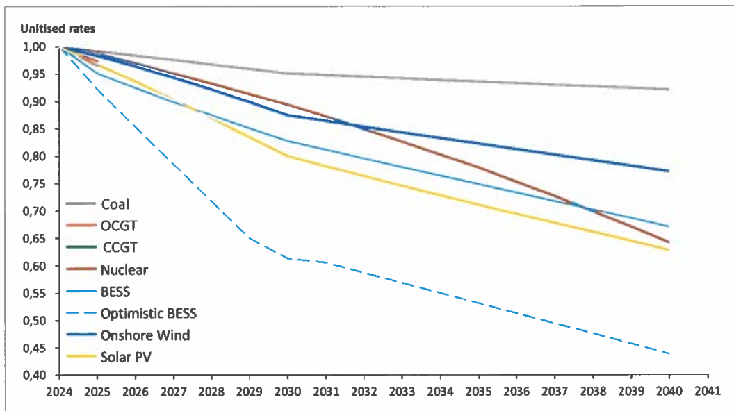
Figure 10: New Technology Cost-Learning Rates.
