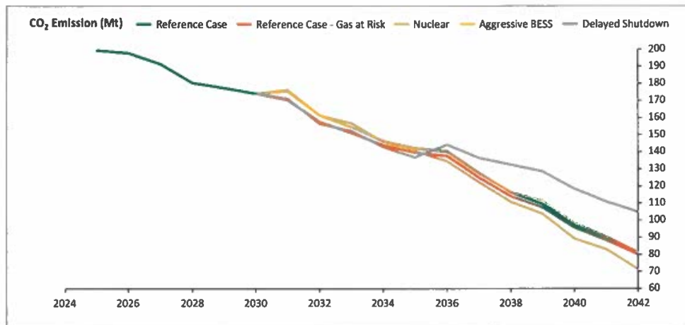
Figure 19: CO 2 Emissions Trajectory (Mt).
