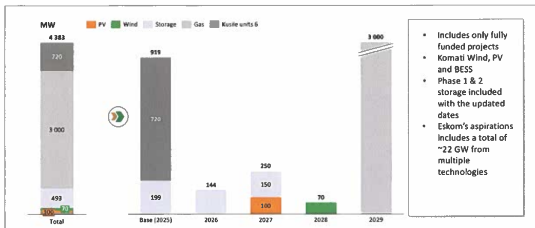
Figure 6: Committed Eskom Generating Capacity.
