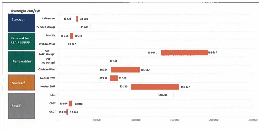
Figure 9: New Technology Cost Assumptions.
