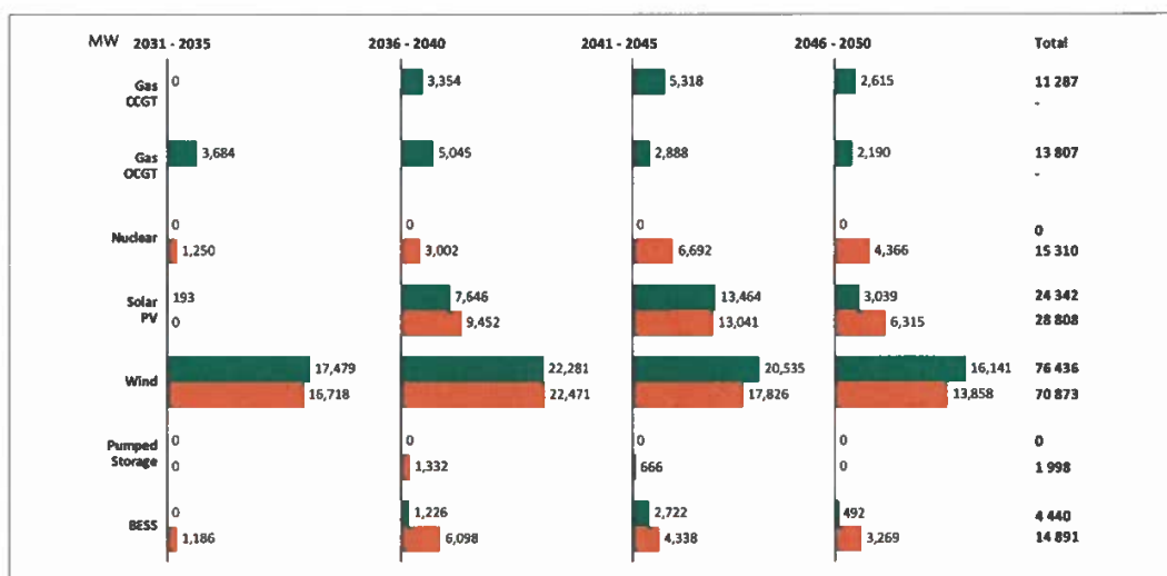
Figure 15: Reference Case and Nuclear.
