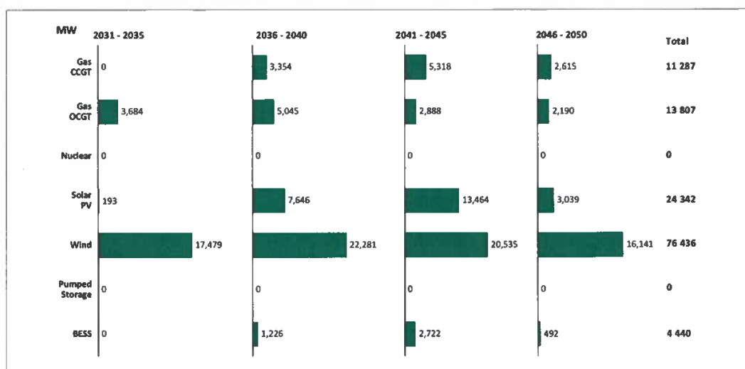
Figure 13: Reference Case Build.
