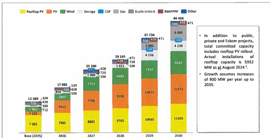
Figure 7: Total Committed Generating Capacity.
