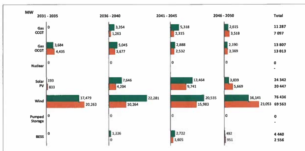
Figure 17: Reference Case and Delayed Coal Shutdown.
